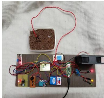
Fig 15 Smart Irrigation system kit
