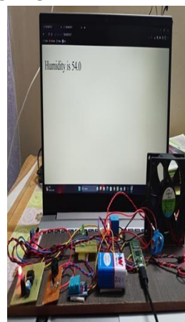
Fig 19 Humidity Output
