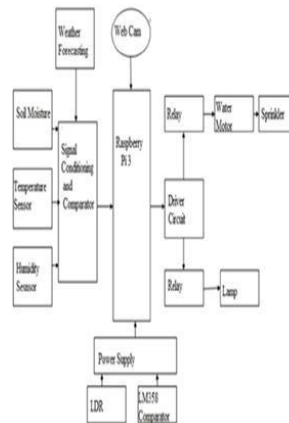
Fig 16. Block diagram
